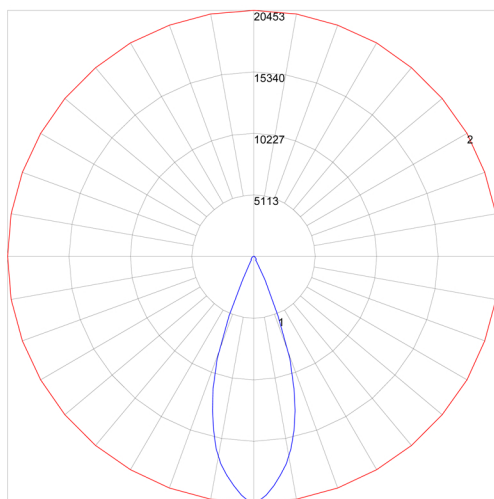
Maximum Candela = 20453 Located At Horizontal Angle = 0, Vertical Angle = 0 # 1 - Vertical Plane Through Horizontal Angles (0 - 180) (Through Max. Cd.) # 2 - Horizontal Cone Through Vertical Angle (0) (Through Max. Cd.)
